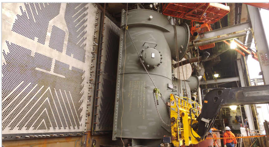
Steam Surface Condenser Modular Changeout
